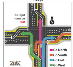
Continuous Flow Intersection 4 Legs
